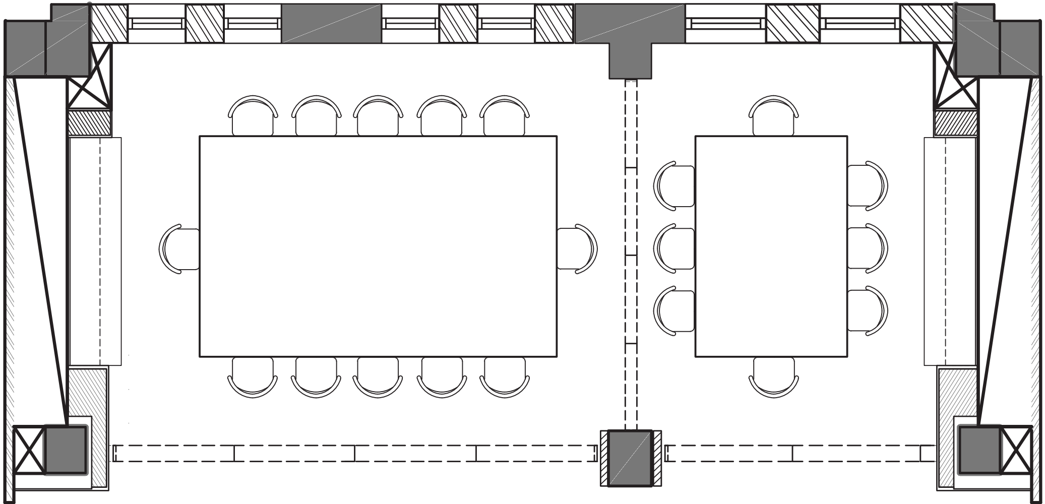
FLOOR PLAN
